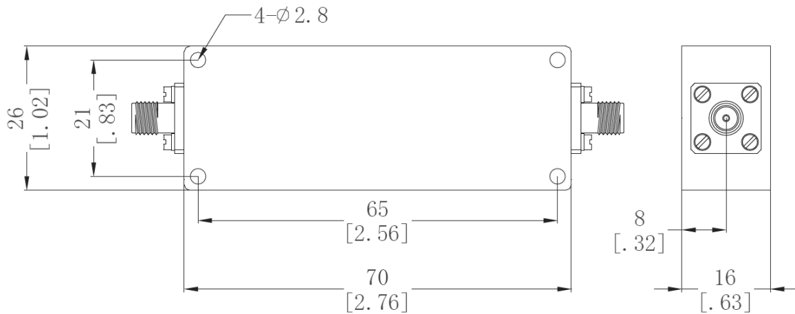
Physical Dimensions ( \pm 0.3\text{mm} )
